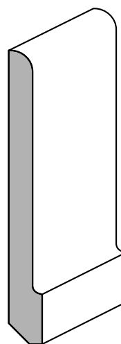
Battiscopa in Ayous mm 70x8x2400
