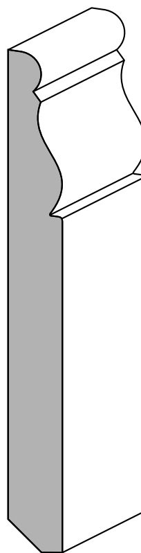
TUDOR Battiscopa in Ayous mm 120x13x2400
