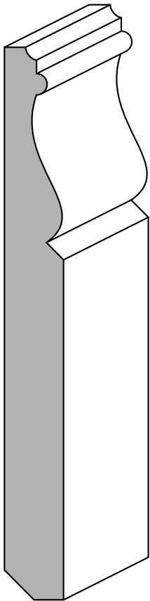
TRADITION Battiscopa in Ayous mm 130x14x2400
