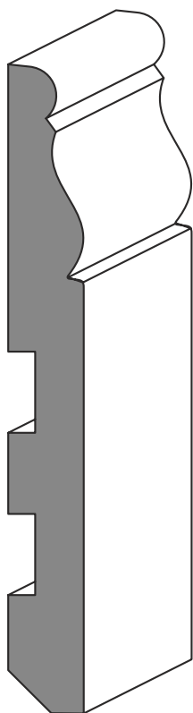
TUDOR Battiscopa in MDF mm 120x14x2200
