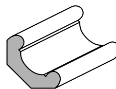
Angolare in Ayous mm 23x10x3000
