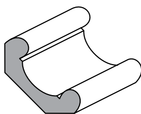
Angolare in Ayous mm 32x12x3000
