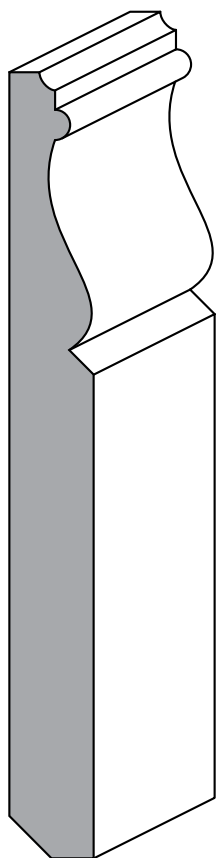
TRADITION Battiscopa in Ayous mm 130x14x2400
