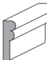
Profilo in Ayous mm 23x7x2000*
